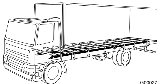
G000276 Fixed body with sub-frame, BAM 1
