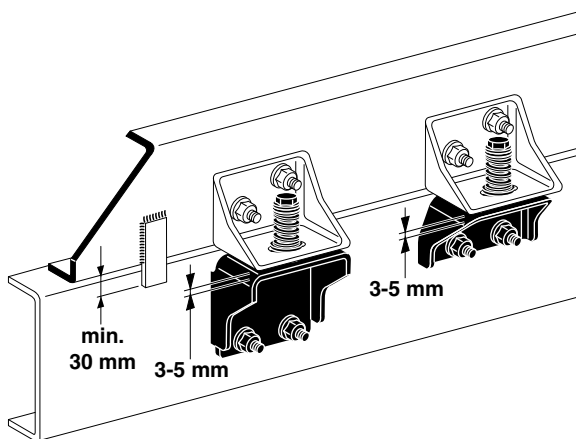
First and second attachment with restrainer plate , LF and CF65 series
